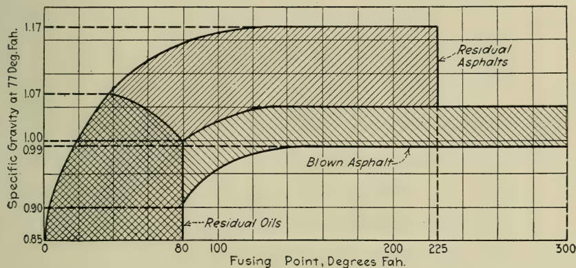
FIG. 112.—Relation between the Specific Gravity and Fusing-Point of Residual Oils, Blown Petroleum Asphalts and Residual Asphalts.
